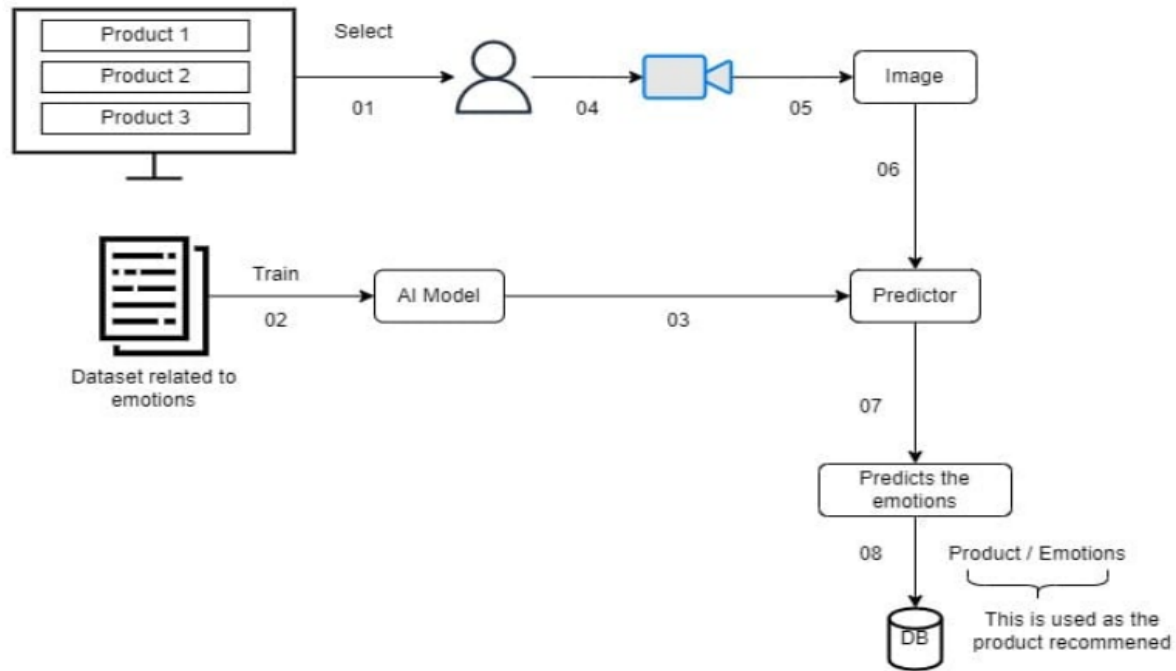
Figure 3: System Architecture
